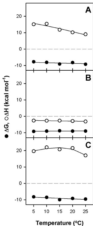
FIGURE 4: Temperature dependence of the apparent binding enthalpy and Gibbs free energy. Experimental values of \Delta H_{app} and \Delta G_{app} at different temperatures for ATP (A) and ADP (B) binding to DnaK T199A and ATP (C) binding to DnaK(1–507) T199A . The temperature dependence of the enthalpy and Gibbs free energy is fitted (solid lines) to the nucleotide binding model described in the Appendix.
