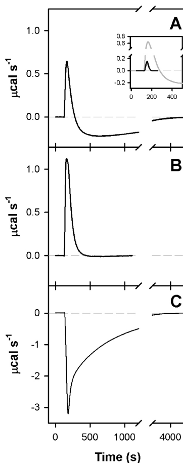
FIGURE 1: ATP binding to DnaK, DnaK T199A , and DnaK R151A (single-injection experiments). Calorimetric traces of a single injection of a stoichiometric concentration of ATP into a solution of DnaK (A), DnaK T199A (B), or DnaK R151A (C). The protein concentration was ca. 20 \mu\text{M} . The experiments were performed in 40 mM Tris-HCl (pH 7.4), 50 mM KCl, and 10 mM MgCl 2 at 25 °C. The inset shows the injection of ATP in buffer under the same experimental conditions.
